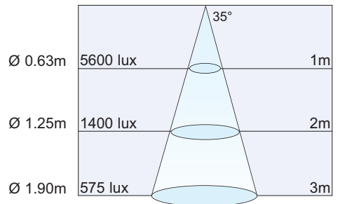
Cool wit 6000K 1800LM
