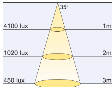
Warm wit 2800K 1300LM
