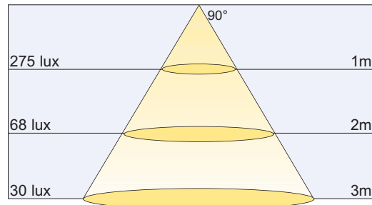
Warm wit 2800K 1450LM
