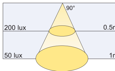
Warm wit 2800K 150LM
