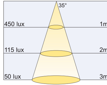
Warm wit 2800K 150LM
